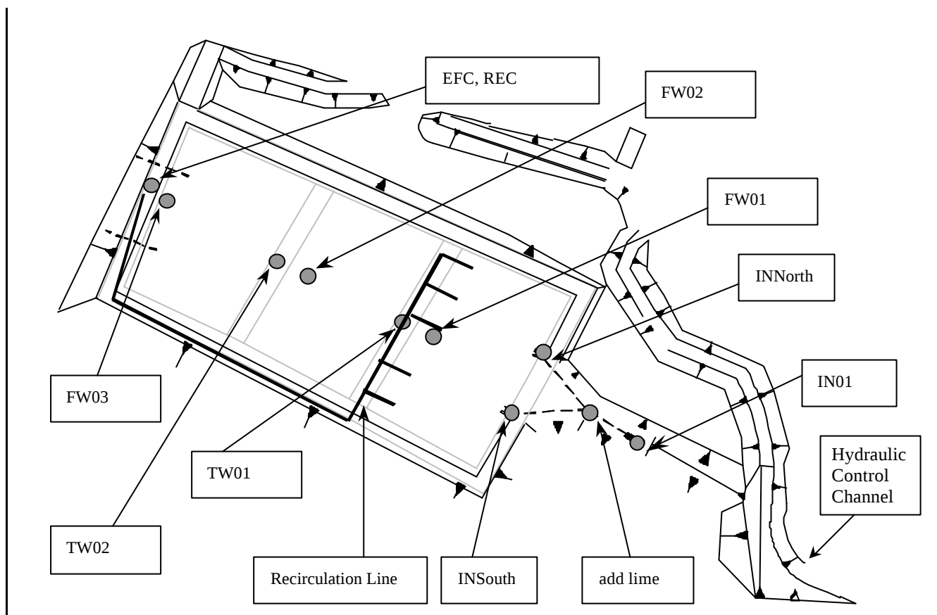
Figure 2. Schematic diagram of Colorado Tailings demonstration wetlands (after Mulholland 1999)
